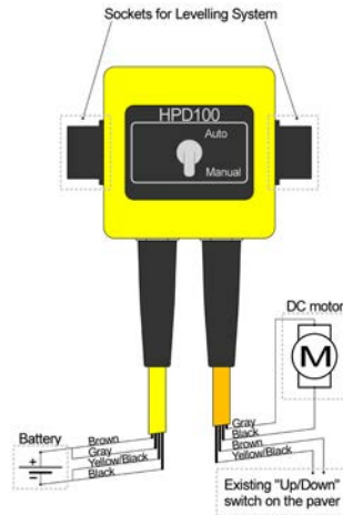
Figure 1 - HPD100 construction
