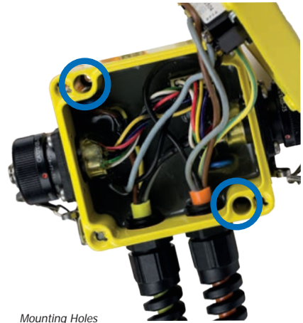
Mounting Holes
