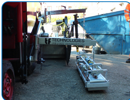
Fig. 4 - Joint Heater Mounted on mounting arms on a machine
